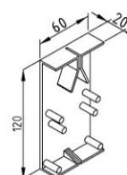
capac HDPE 60 lamele X121,2F
